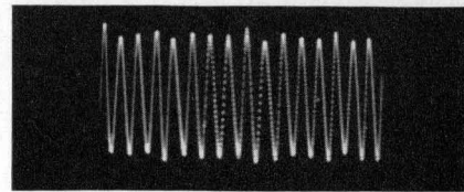
Fig. 4. Oscillogram obtained when using generator to investigate screeching shaft. Screech vibrations are evidenced by breaks in otherwise continuous waveform.
